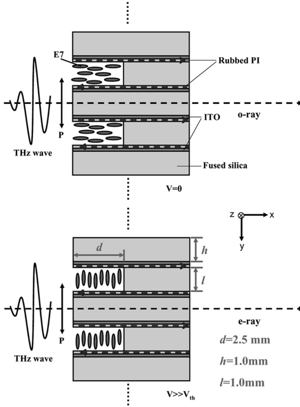
FIGURE 2 Schematic illustration of electrically controlled NLC based THz phase grating. The polarization and propagation direction of incident THz wave are parallel to y- and x-axis, respectively. The director of NLC is rotated from x- to y-axis with increasing applied bias. ITO: indium-tin-oxide film as electrode, P: polarization of THz wave, V: bias, V_{th} : threshold voltage. The dimensions of the structure are shown.
